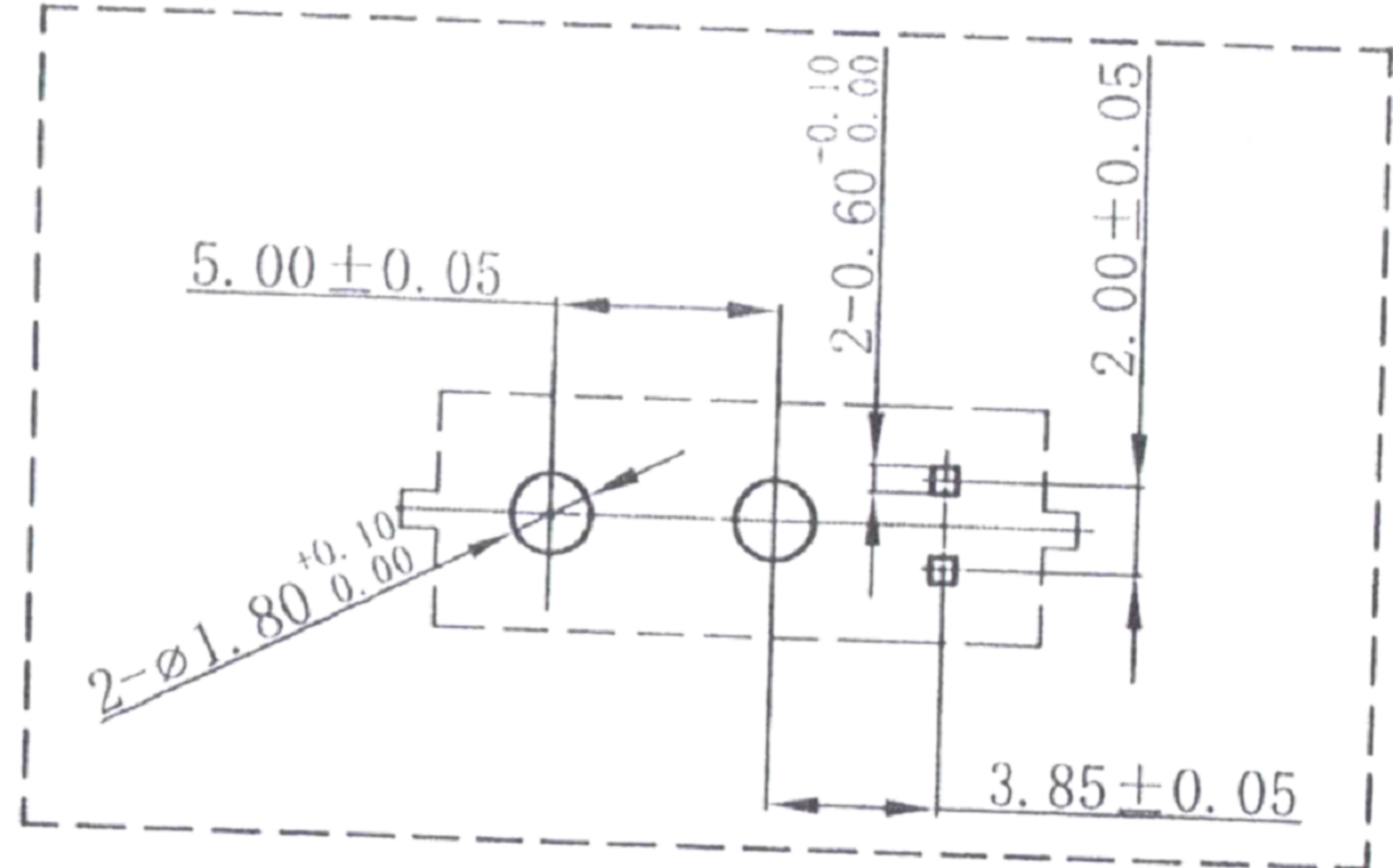
PCB LAYOUT
